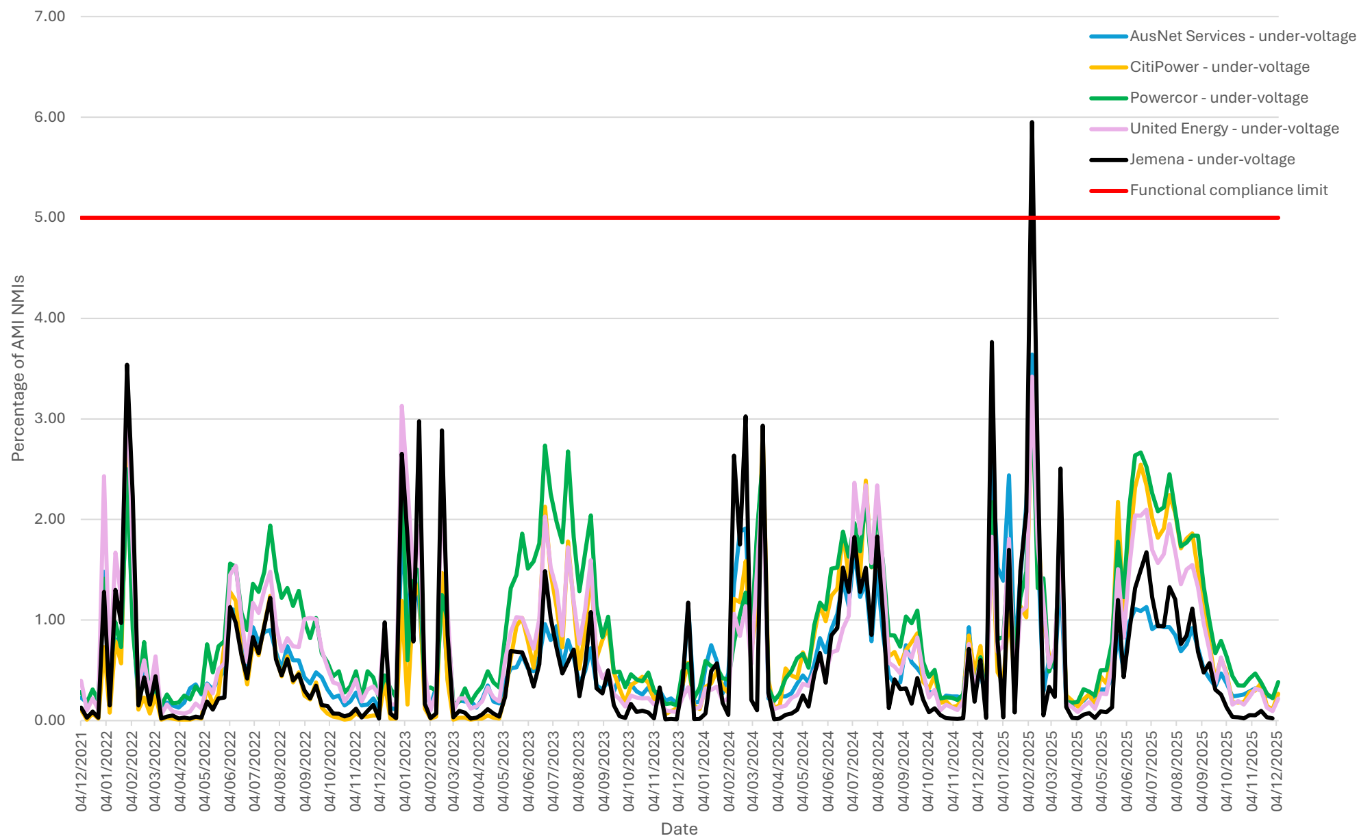
Graph 2: % of NMI's below 216V for more than 1% of the time (under-voltage)
