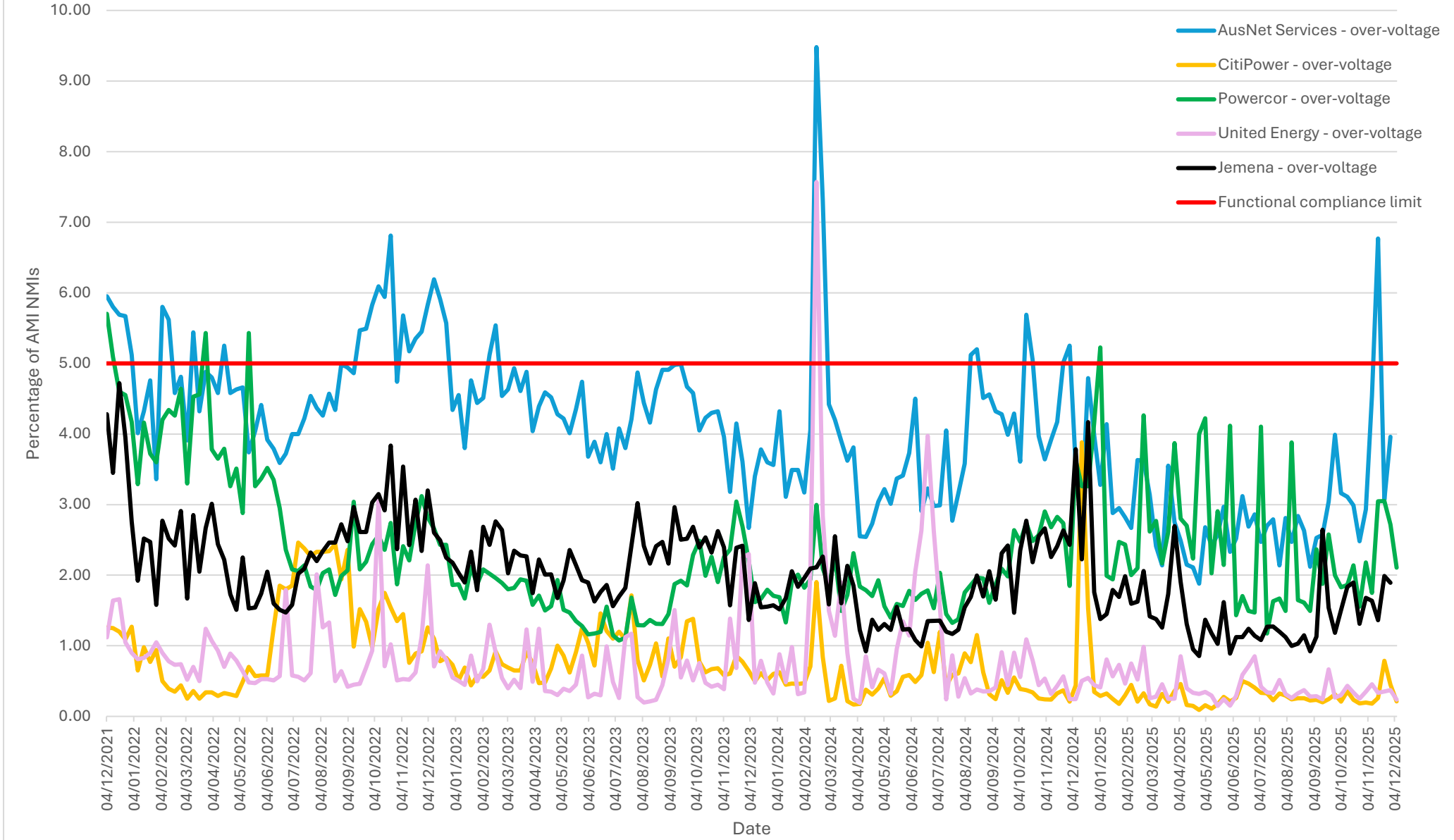
Graph 1: % of NMIs above 253V for more than 1% of the time (over-voltage)
