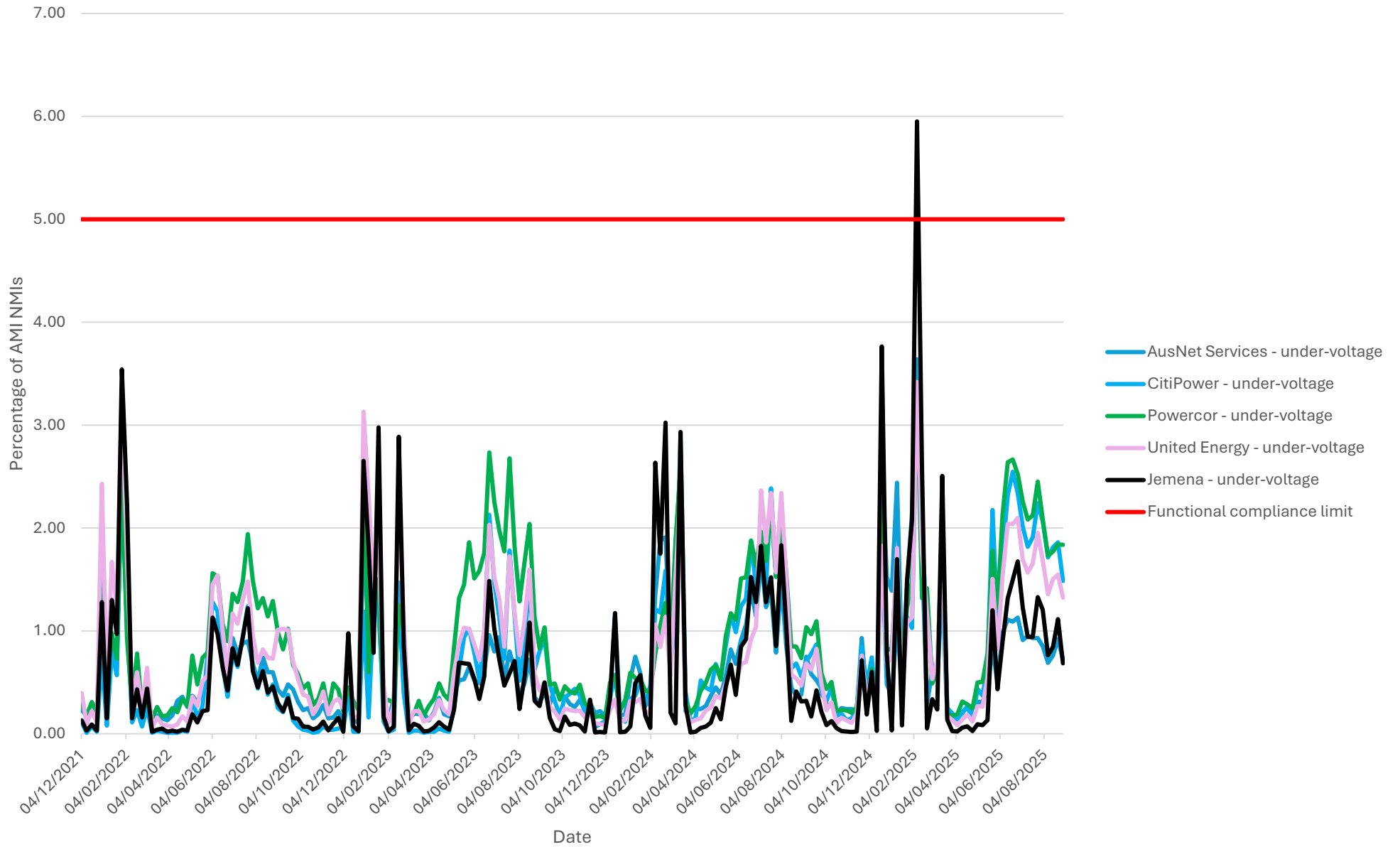
Graph 2: % of NMI below 216V for more than 1% of the time (under-voltage)
